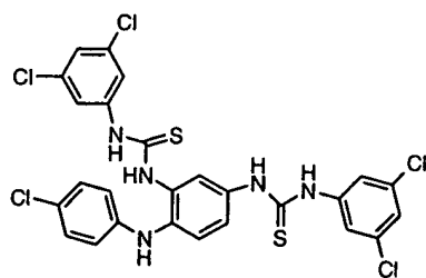
Compound # 36
